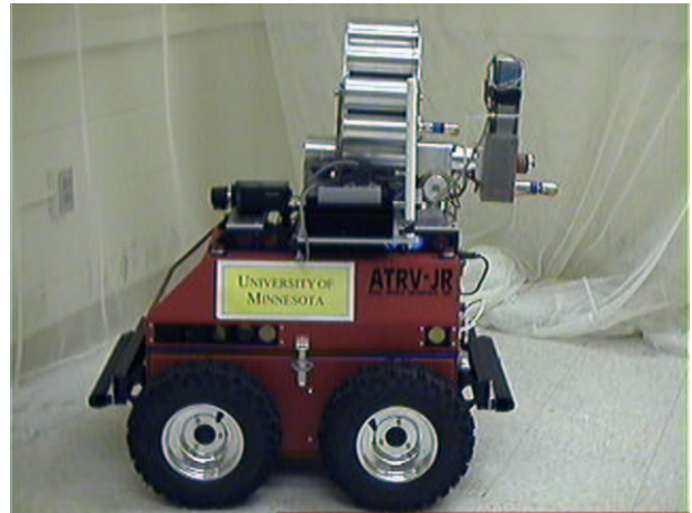
Figure 2: A ranger robot with scout launcher.
