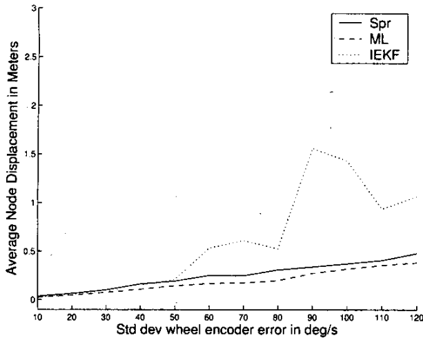
Fig. 6. Comparison of the means and standard deviations of the three estimators on datasets with varying degrees of encoder error. Standard deviation of errors ranged from 10 deg/sec to 120 deg/sec.
