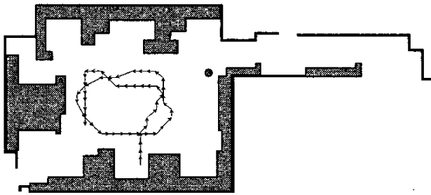
Fig. 4. The path of the robot through the office environment.
