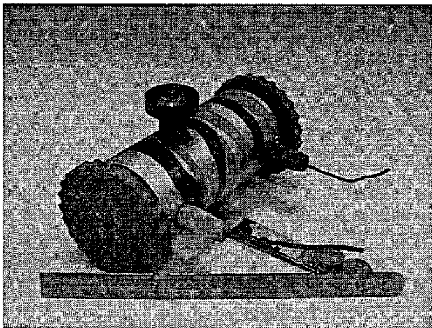
Fig. 1. A Scout robot with an upward-facing Omnittech 190° fisheye lens. The lens provides 360° horizontal field of view around the robot, effectively functioning as an omnicaamera. The robot is 11 cm long and 4 cm in diameter.
